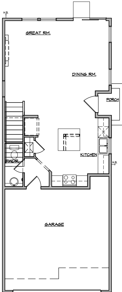
MAIN FLOOR PLAN ('A', 'B' & 'C' SIM)
